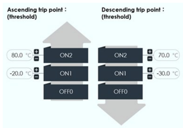
Figure 3-11-1 Temperature Input Threshold
