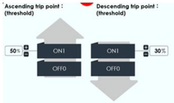
Figure 3-19: PWM input thresholds
