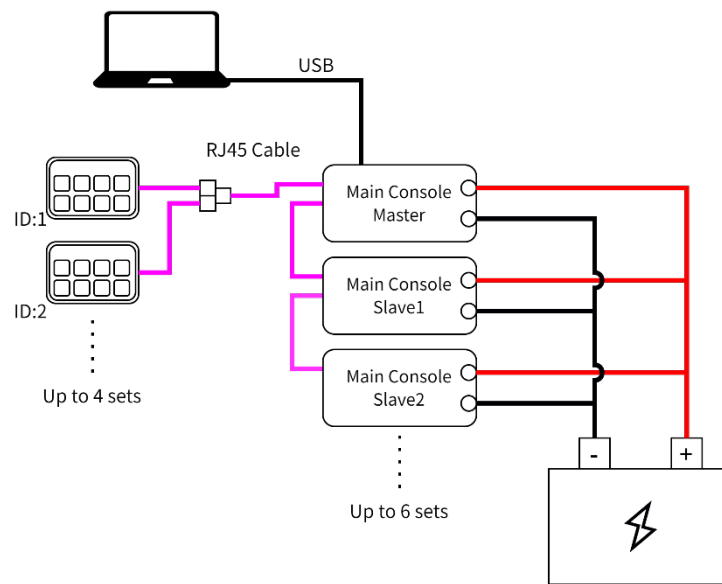
Figure 1-3-1 AXIXLINK High-Level Architecture
