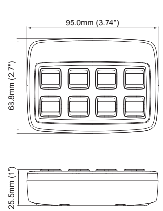
Controller
